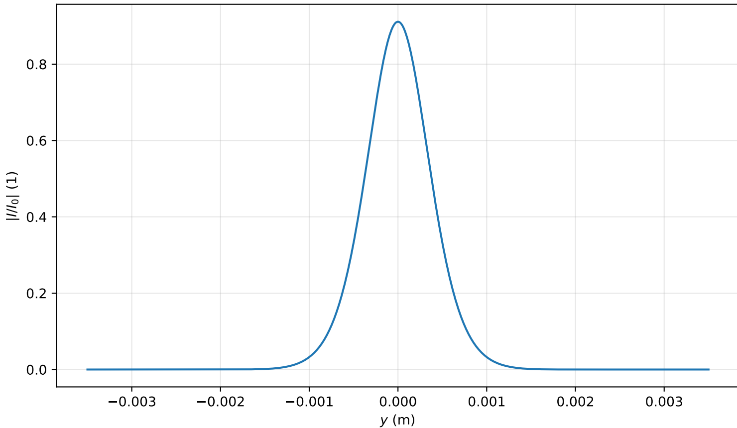
Intensity profile I(x=0, y, z=1.353)/I_0 , P_{in}=0.4P_{cr} , artificial time
